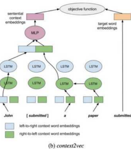
Figure 1: word2vec and context2vec architectures.
